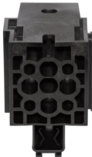
Socket waterproof incl. metal bracket and silicone gasket
